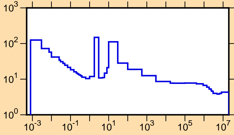
\sigma vs. E for ^{107}\text{In}(n,\text{tot.})
