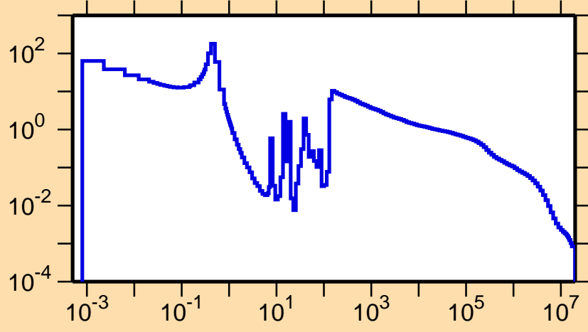
\sigma vs. E for ^{108}\text{In}(n,\gamma)
