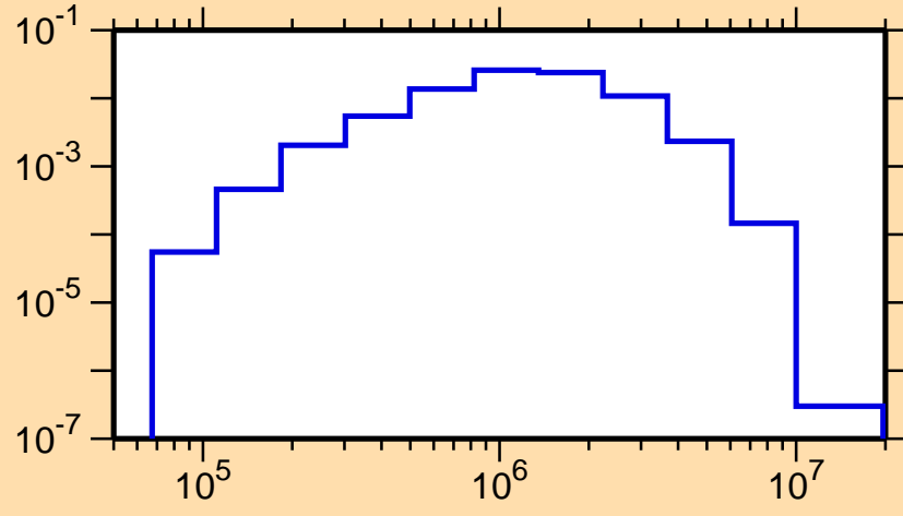
\sigma vs. E for ^{108}\text{In}(n, n_2)
