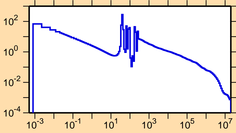
\sigma vs. E for ^{109}\text{In}(n,\gamma)
