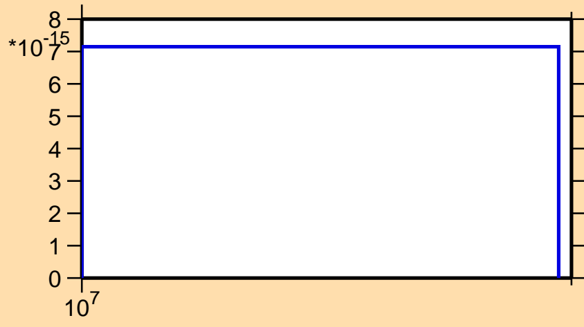
\sigma vs. E for ^{109}\text{In}(n,\text{pt})
