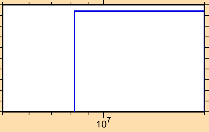
\sigma vs. E for ^{109}\text{In}(n,nt)
