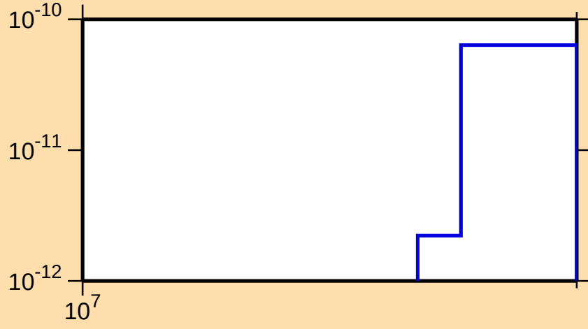
\sigma vs. E for ^{110}\text{In}(\text{mt117})
