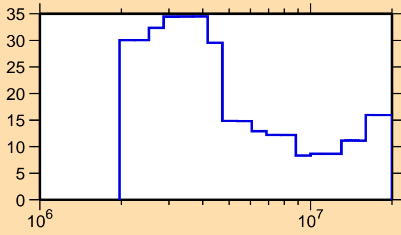
\Delta\sigma/\sigma vs. E for ^{111}\text{In}(n, el.)
