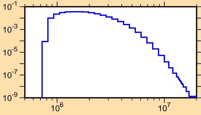
\sigma vs. E for ^{111}\text{In}(n,n_2)
