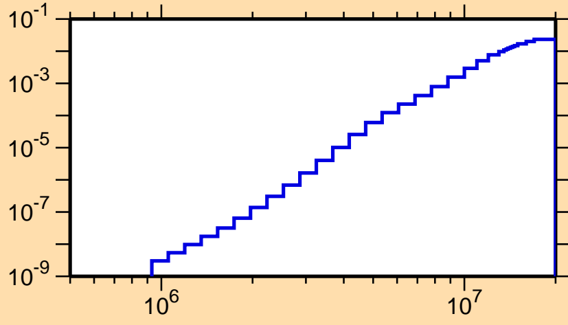
\sigma vs. E for ^{111}\text{In}(n,\alpha)
