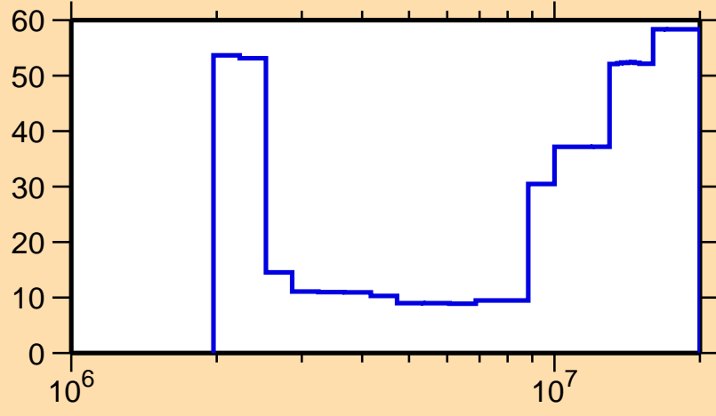
\Delta\sigma/\sigma vs. E for ^{111}\text{In}(n,n\text{cont.})
