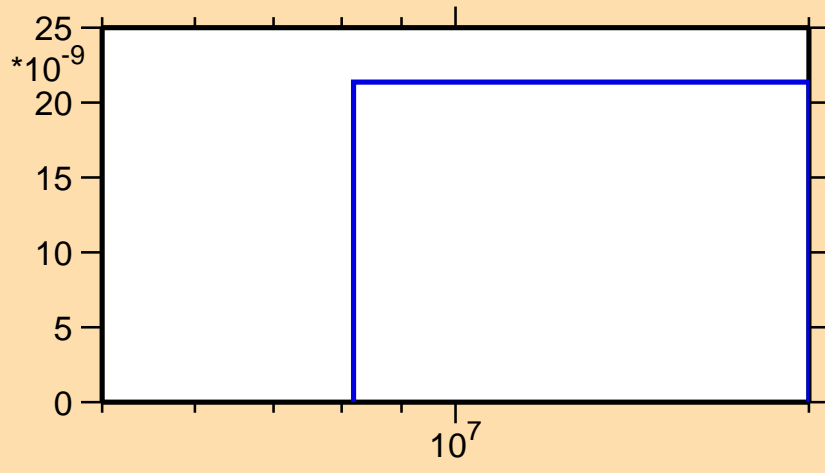
\sigma vs. E for ^{111}\text{In}(n,p\alpha)
