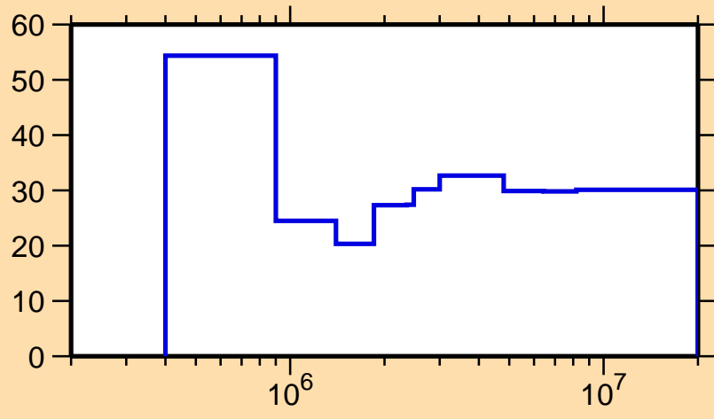
\Delta\sigma/\sigma vs. E for ^{111}\text{In}(n,n_1)
