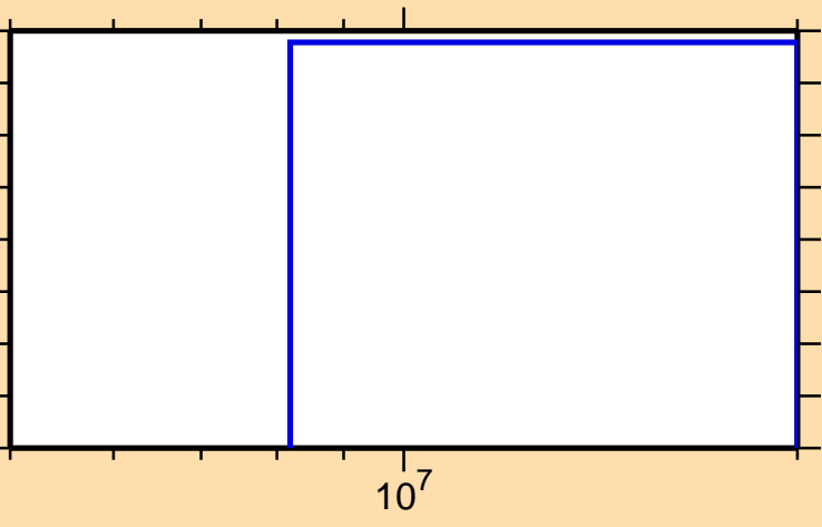
\sigma vs. E for ^{111}\text{In}(n,\text{nd})
