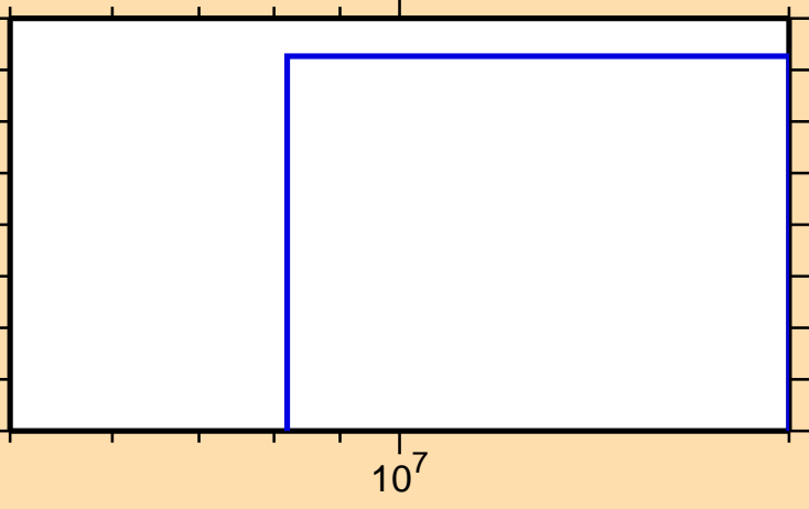
\sigma vs. E for ^{111}\text{In}(n,3n)
