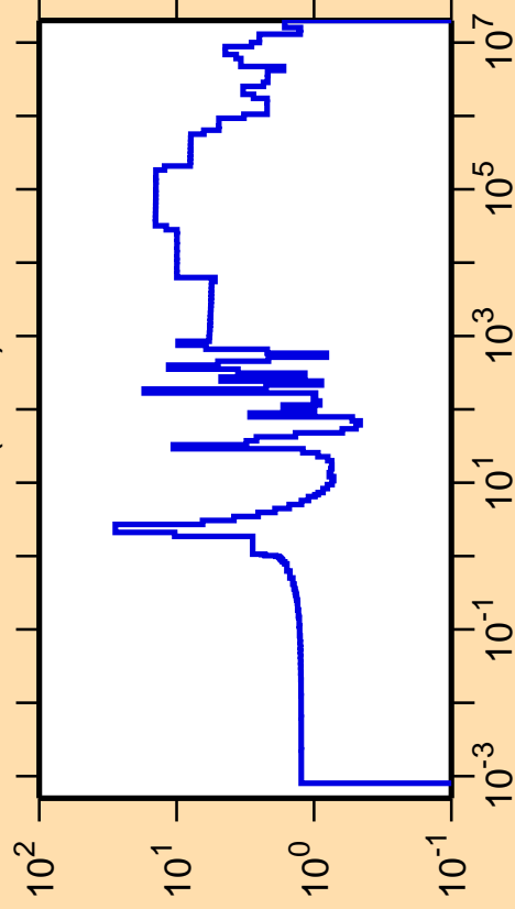
\Delta\sigma/\sigma vs. E for ^{111}\text{In}(n,\text{el.})
