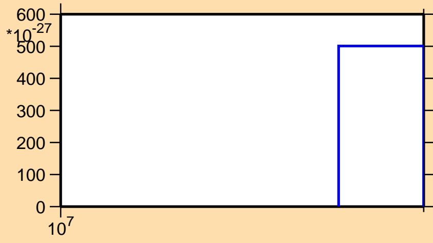
\sigma vs. E for ^{111}\text{In} (mt 11)
