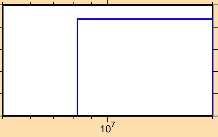
\sigma vs. E for ^{111}\text{In}(n,\text{pd})
