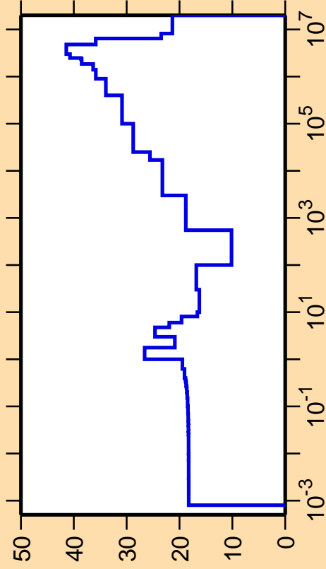
\Delta\sigma/\sigma vs. E for ^{111}\text{In}(\text{n},\gamma)
