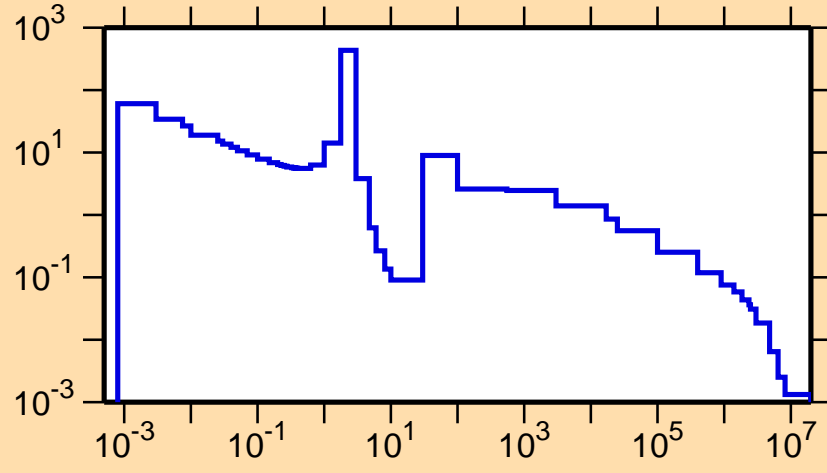
\sigma vs. E for ^{111}\text{In}(\text{n},\gamma)
