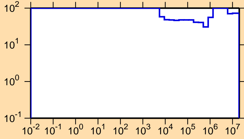
\Delta\sigma/\sigma vs. E for ^{112}\text{In}(n,p)
