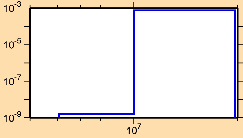
\sigma vs. E for ^{112}\text{In}(n,\alpha)
