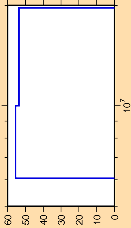
\Delta\sigma/\sigma vs. E for ^{112}\text{In}(n,\alpha)
