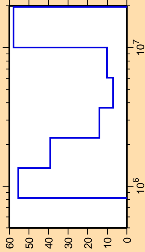
\Delta\sigma/\sigma vs. E for ^{112}\text{In}(n,n\text{cont.})
