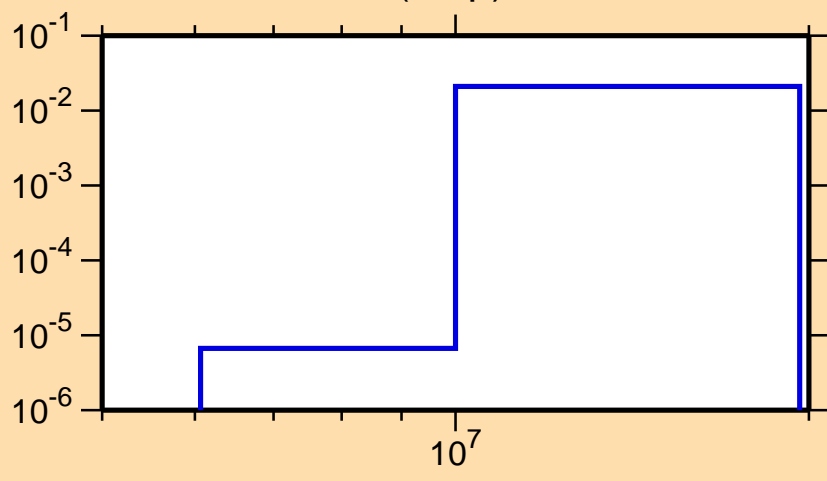
\sigma vs. E for ^{112}\text{In}(n,np)
