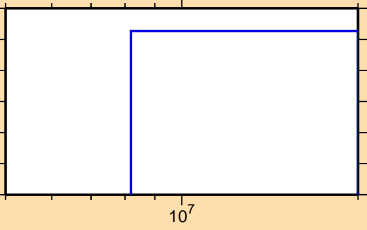
\sigma vs. E for ^{113}\text{In}(n,t)
