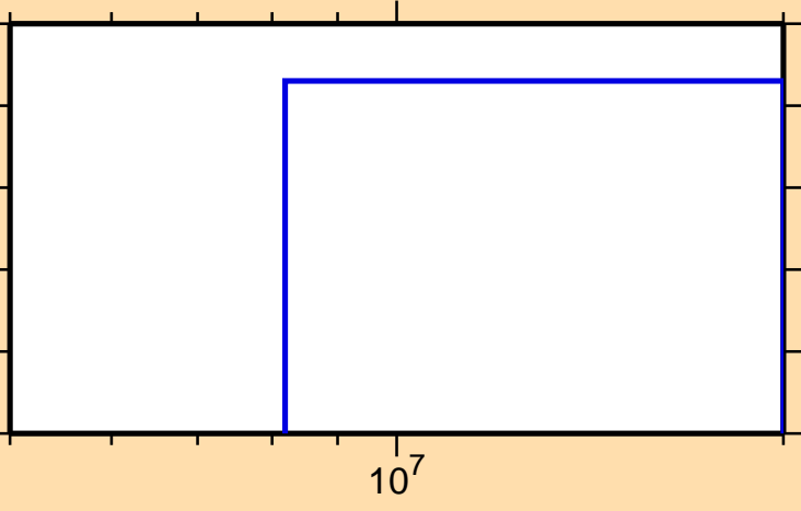
\sigma vs. E for ^{113}\text{In}(n,2np)
