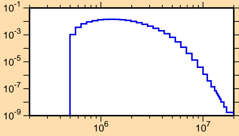
\sigma vs. E for ^{114}\text{In}(n,n_4)
