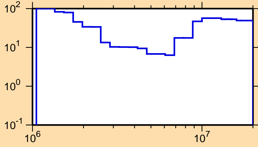
\Delta\sigma/\sigma vs. E for ^{114}\text{In}(n,n\text{cont.})
