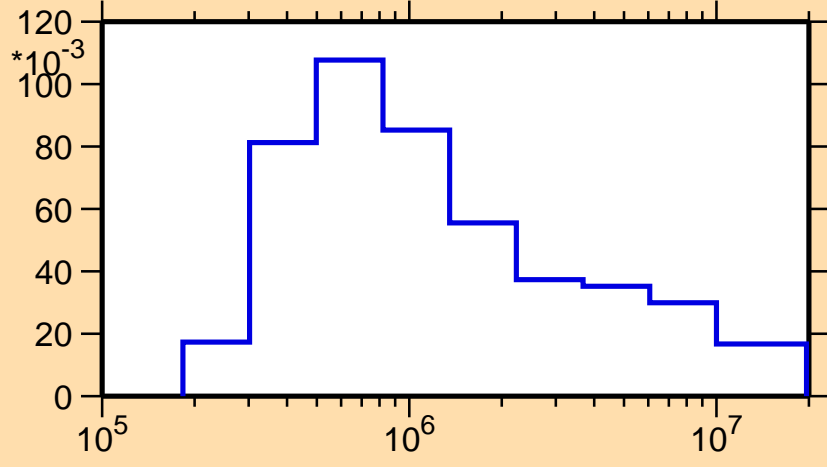
\sigma vs. E for ^{114}\text{In}(n,n_2)
