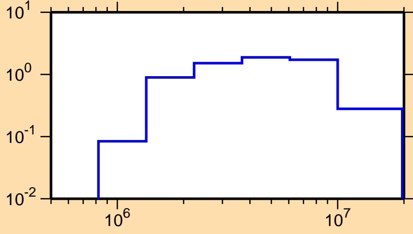
\sigma vs. E for ^{114}\text{In}(n,n\text{cont.})
