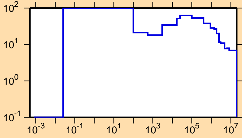
\Delta\sigma/\sigma vs. E for ^{114}\text{In}(n,\text{nonel.})
