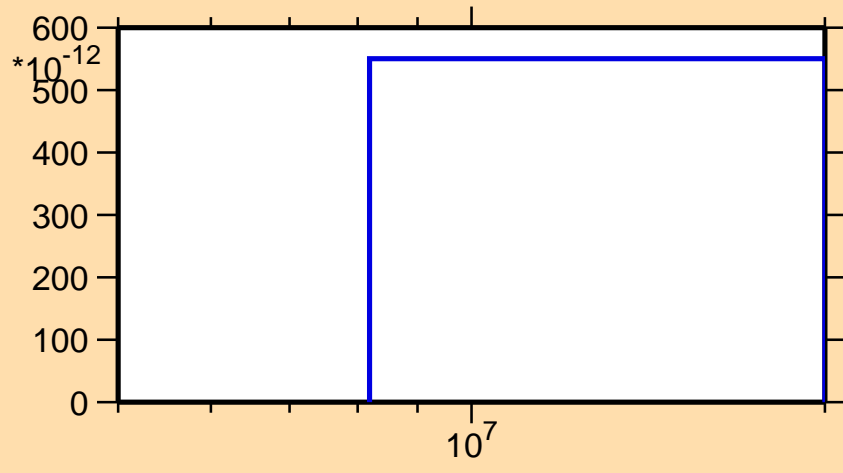
\sigma vs. E for ^{114}\text{In}(n,p\alpha)
