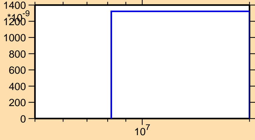
\sigma vs. E for ^{114}\text{In}(n,2np)
