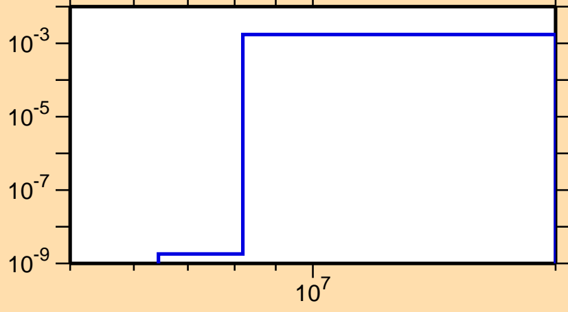
\sigma vs. E for ^{114}\text{In}(n,d)
