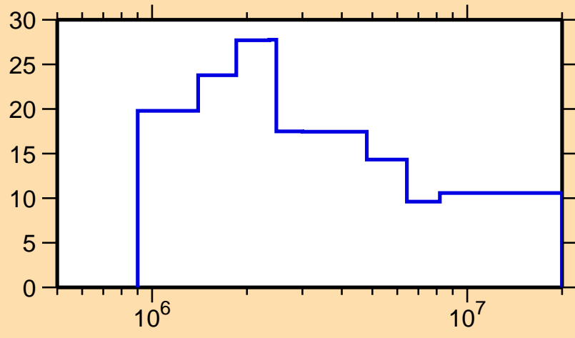
\Delta\sigma/\sigma vs. E for ^{114}\text{In}(n, el.)
