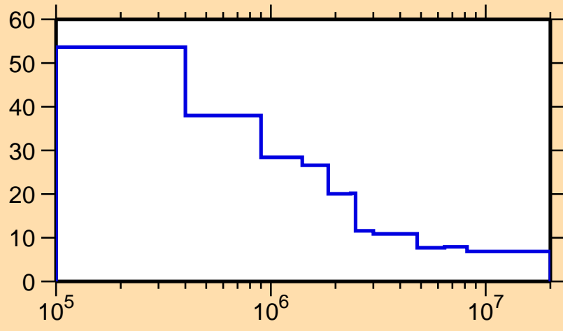
\Delta\sigma/\sigma vs. E for ^{114}\text{In}(n,\text{nonel.})
