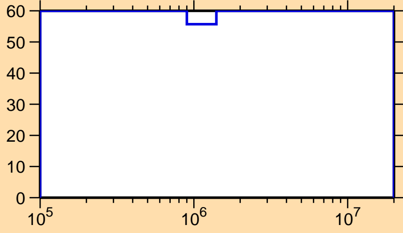
\Delta\sigma/\sigma vs. E for ^{114}\text{In}(n,n_1)
