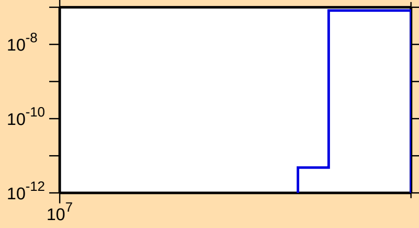
\sigma vs. E for ^{114}\text{In}(n,nt)
