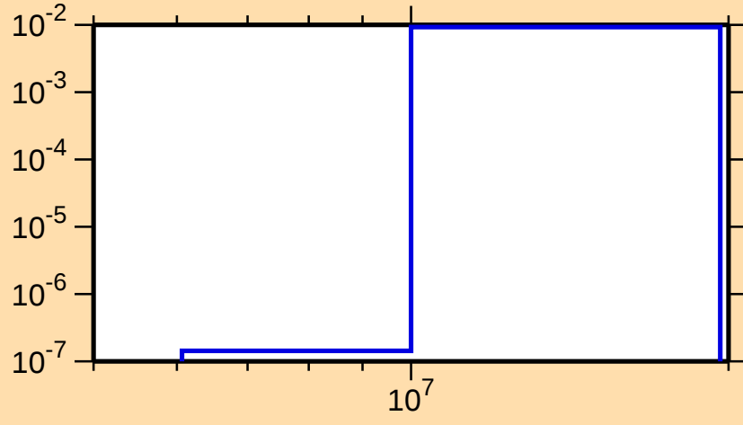
\sigma vs. E for ^{114}\text{In}(n,np)
