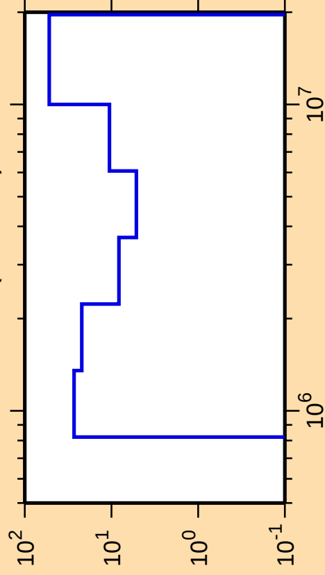
\Delta\sigma/\sigma vs. E for ^{114}\text{In}(n,n\text{cont.})
