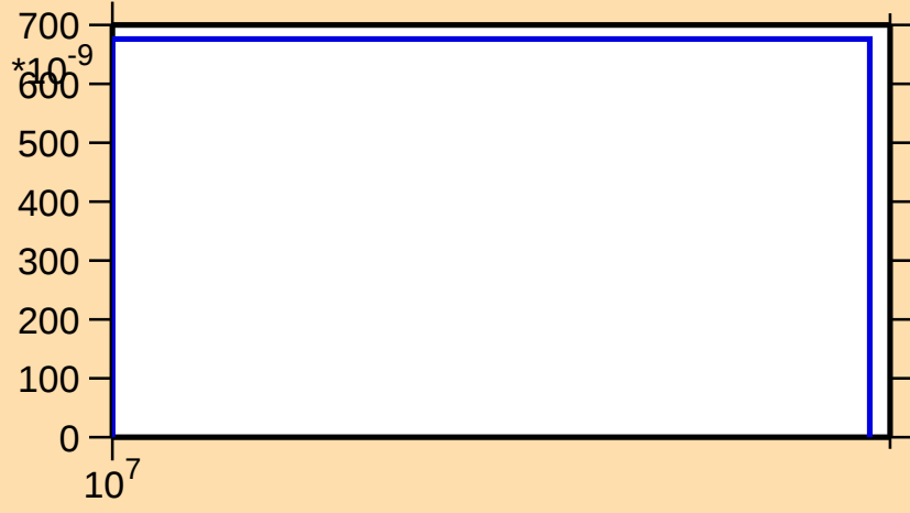
\sigma vs. E for ^{114}\text{In}(n,\text{nd})
