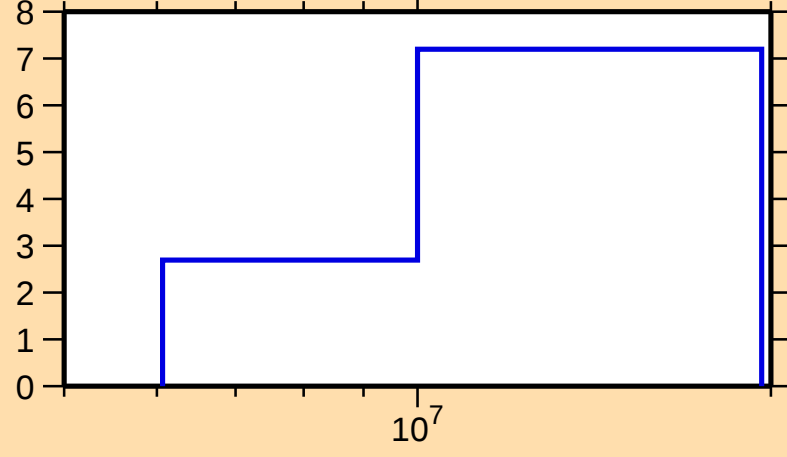
\Delta\sigma/\sigma vs. E for ^{114}\text{In}(n,\text{tot.})
