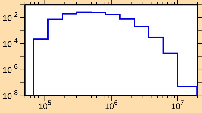
\sigma vs. E for ^{114}\text{In}(n,n_3)
