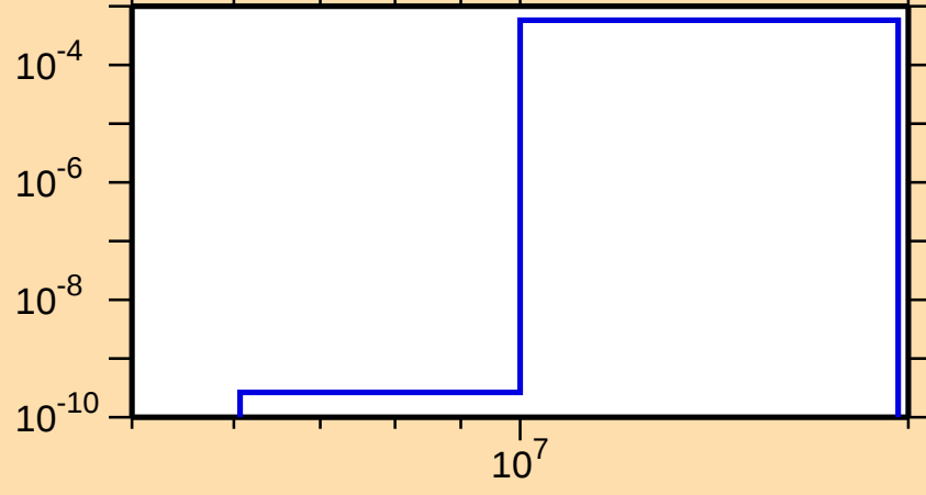
\sigma vs. E for ^{114}\text{In}(n,t)
