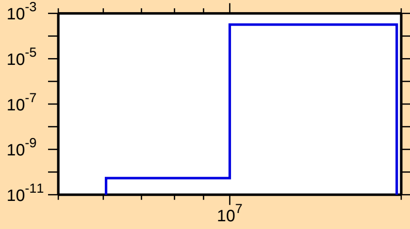
\sigma vs. E for ^{114}\text{In}(n,n\alpha)
