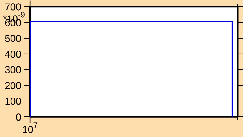
\sigma vs. E for ^{114}\text{In}(n,2np)
