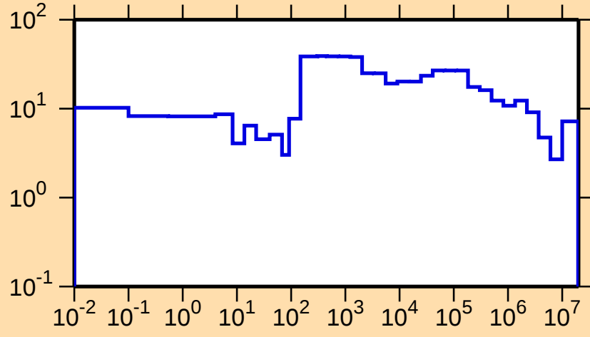
\Delta\sigma/\sigma vs. E for ^{114}\text{In}(n,\text{tot.})
