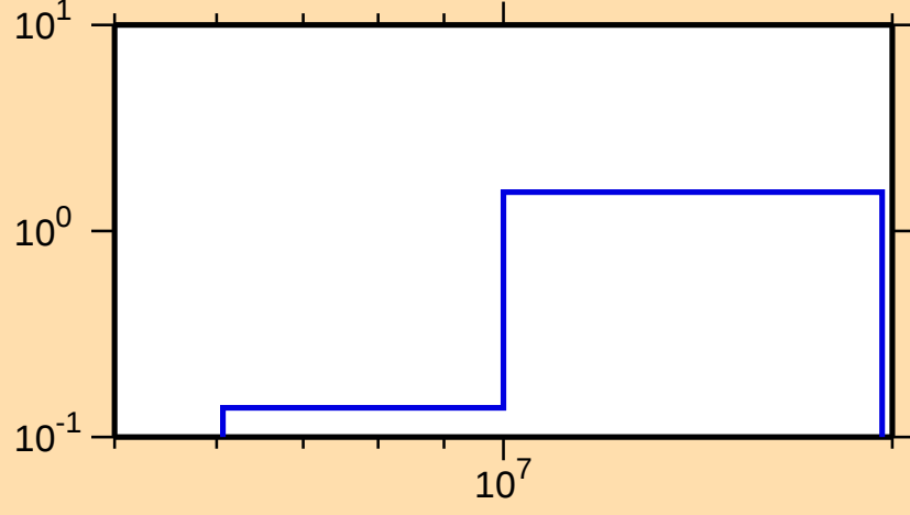
\sigma vs. E for ^{114}\text{In}(n,2n)
