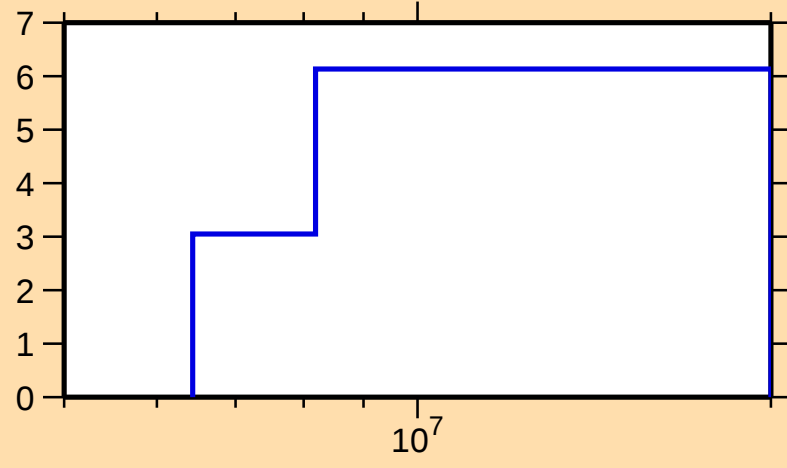
\Delta\sigma/\sigma vs. E for ^{114}\text{In}(n,\text{tot.})
