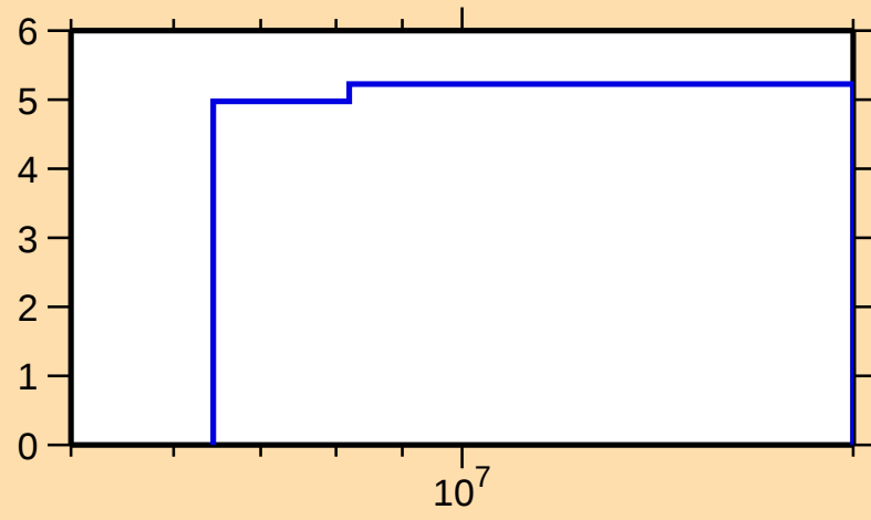
\Delta\sigma/\sigma vs. E for ^{114}\text{In}(n,\text{nonel.})
