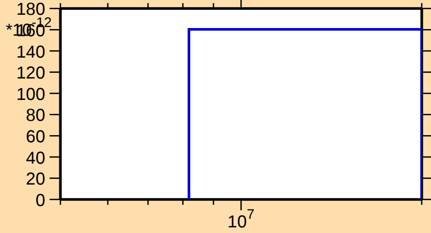
\sigma vs. E for ^{114}\text{In}(n,p\alpha)
