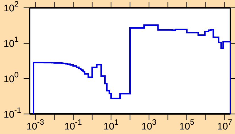
\Delta\sigma/\sigma vs. E for ^{114}\text{In}(n,\text{el.})
