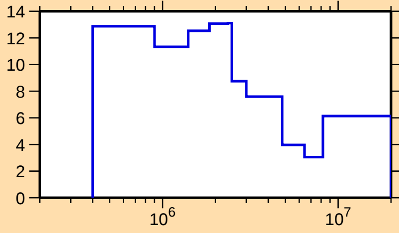
\Delta\sigma/\sigma vs. E for ^{114}\text{In}(n,\text{tot.})
