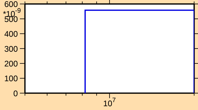
\sigma vs. E for ^{114}\text{In}(n,\text{nd})
