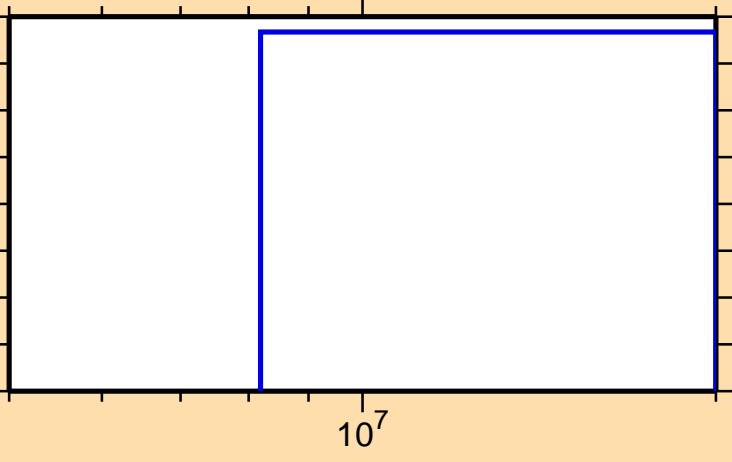
\sigma vs. E for ^{115}\text{In}(n,p\alpha)
