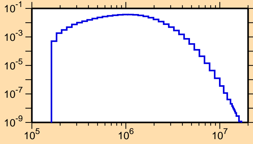
\sigma vs. E for ^{116}\text{In}(n,n_4)
