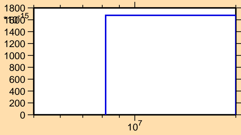
\sigma vs. E for ^{116}\text{In}(n,p\alpha)
