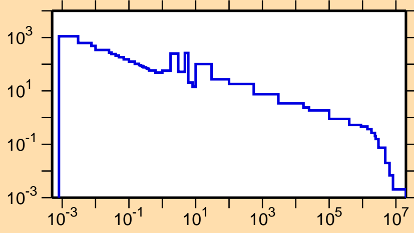
\sigma vs. E for ^{116}\text{In}(n,\gamma)
