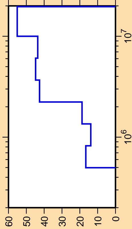
\Delta\sigma/\sigma vs. E for ^{117}\text{In}(n,n_2)
