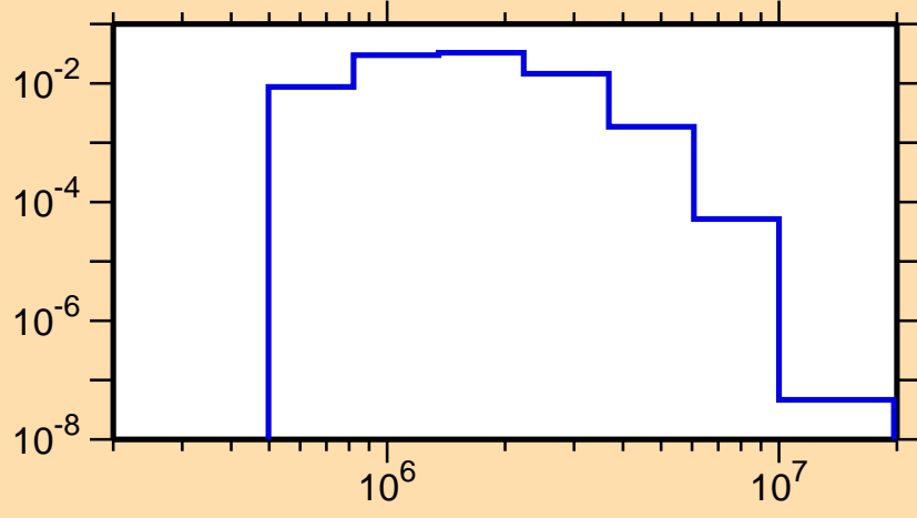
\sigma vs. E for ^{117}\text{In}(n,n_2)
