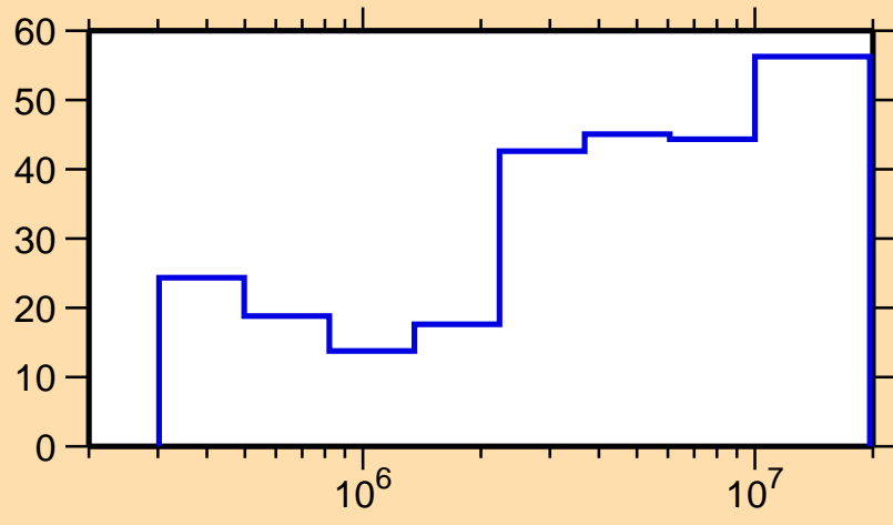
\Delta\sigma/\sigma vs. E for ^{117}\text{In}(n,n_1)
