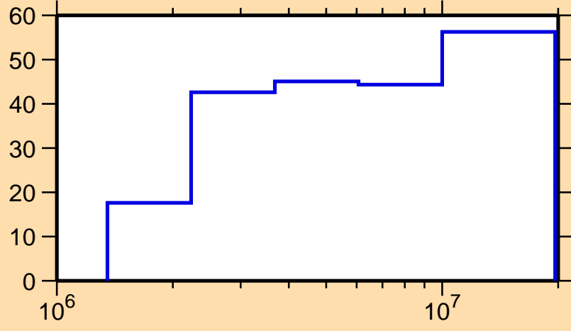
\Delta\sigma/\sigma vs. E for ^{117}\text{In}(n, n_1)
