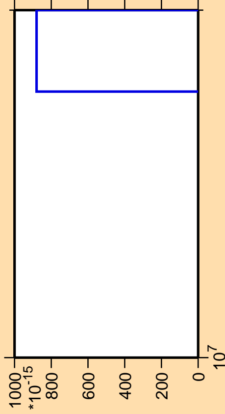
\Delta\sigma/\sigma vs. E for ^{117}\text{In} (mt 11)
