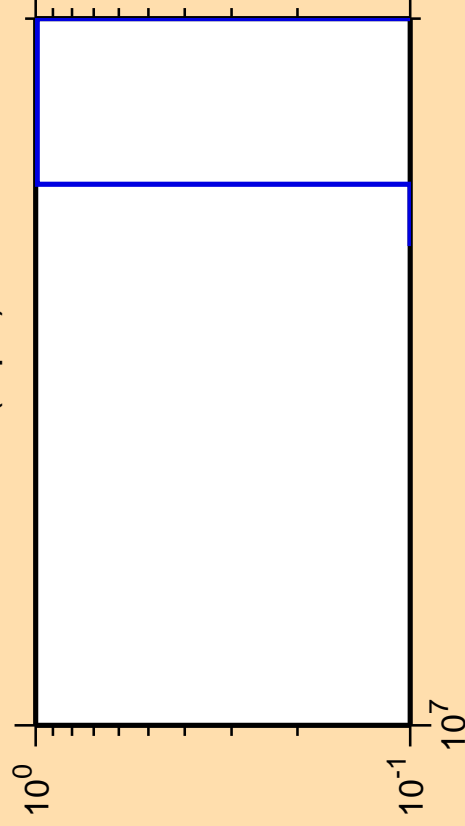
\Delta\sigma/\sigma vs. E for ^{117}\text{In}(n,p\alpha)
