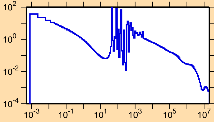
\sigma vs. E for ^{117}\text{In}(n,\gamma)
