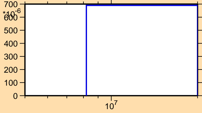
\sigma vs. E for ^{118}\text{In}(n,np)
