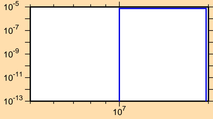
\sigma vs. E for ^{118}\text{In}(n,\alpha)
