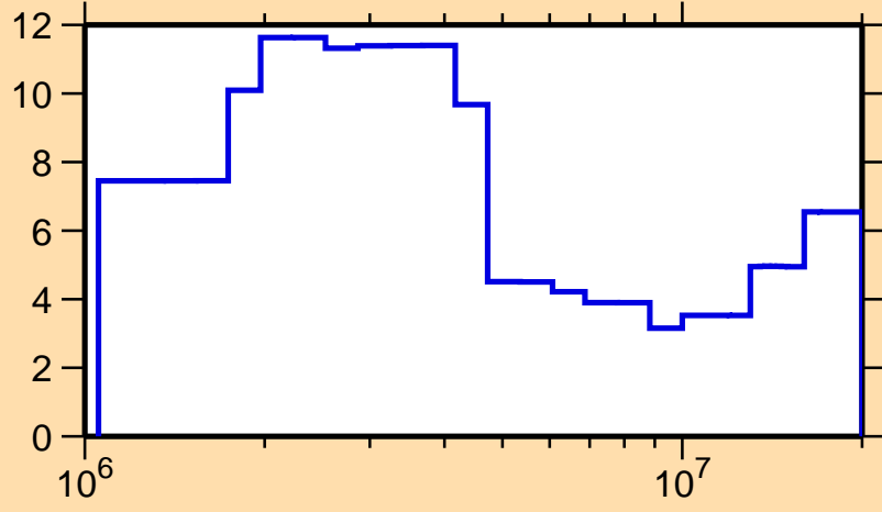
\Delta\sigma/\sigma vs. E for ^{118}\text{In}(n, el.)
