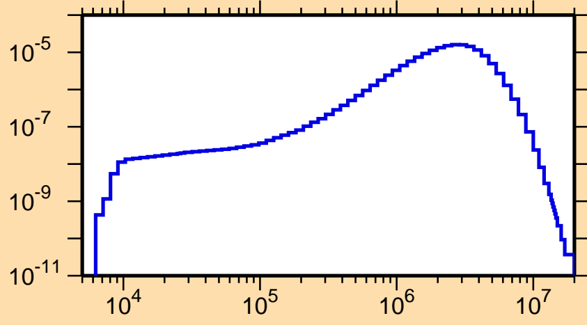
\sigma vs. E for ^{120}\text{In}(n,n_1)
