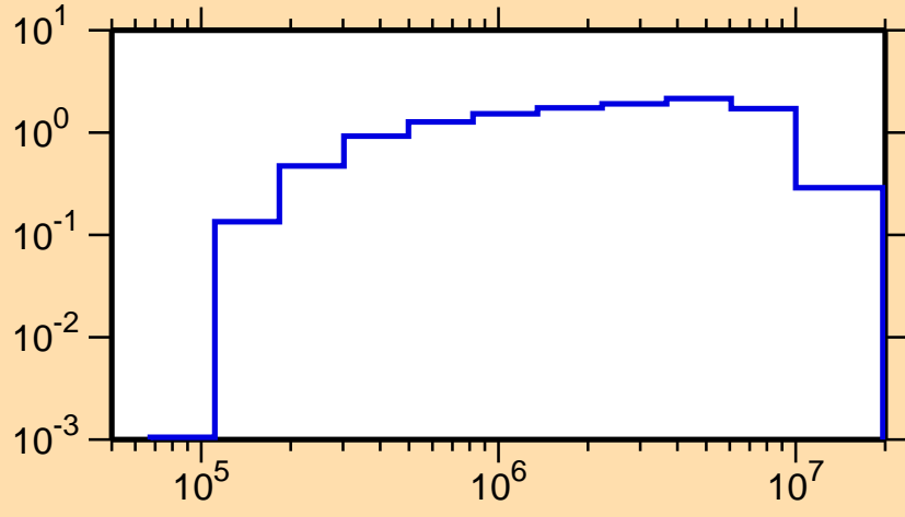
\sigma vs. E for ^{120}\text{In}(n,n\text{cont.})
