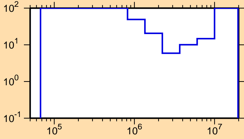
\Delta\sigma/\sigma vs. E for ^{120}\text{In}(n,n\text{cont.})
