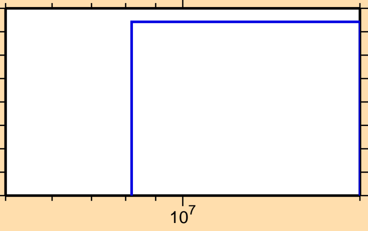
\sigma vs. E for ^{120}\text{In}(n,d)
