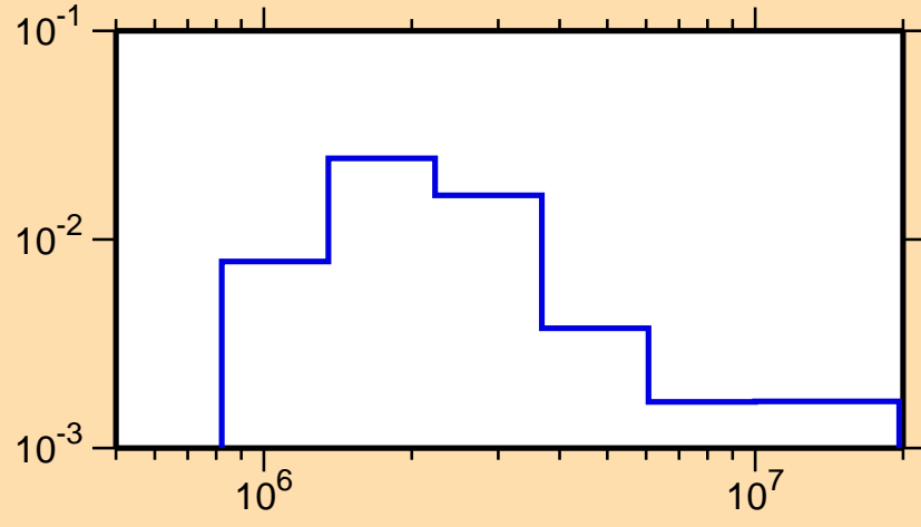
\sigma vs. E for ^{121}\text{In}(n,n_3)
