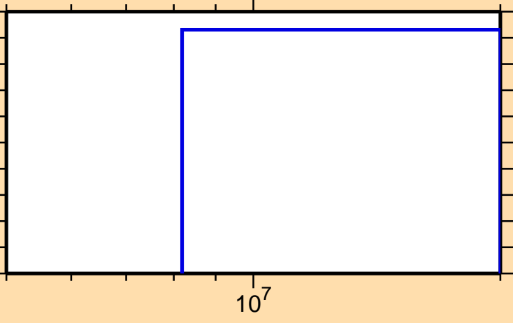
\sigma vs. E for ^{121}\text{In}(n,t)
