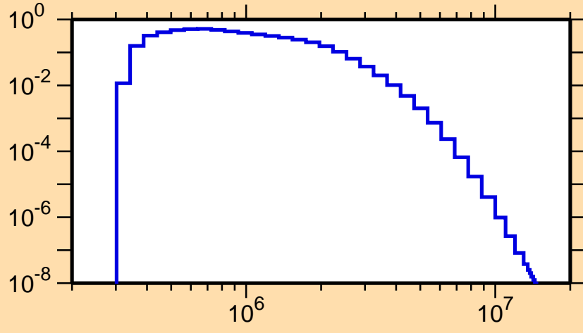
\sigma vs. E for ^{121}\text{In}(n,n_2)
