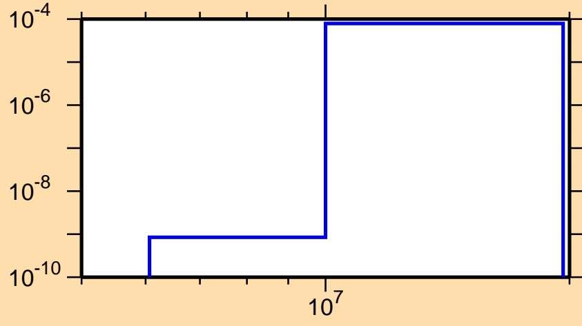
\sigma vs. E for ^{121}\text{In}(n,\alpha)
