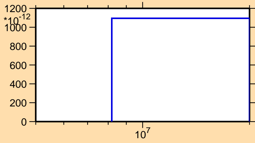
\sigma vs. E for ^{121}\text{In}(n,nt)
