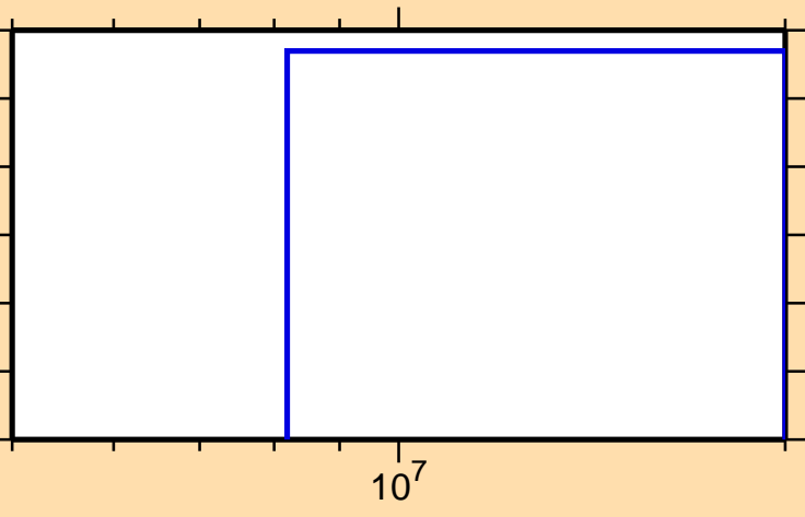
\sigma vs. E for ^{121}\text{In}(n,\alpha)
