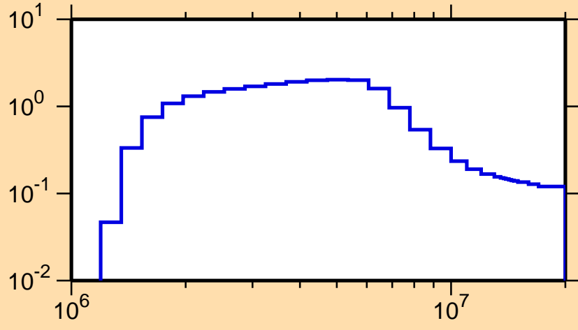
\sigma vs. E for ^{122}\text{In}(n,n\text{cont.})
