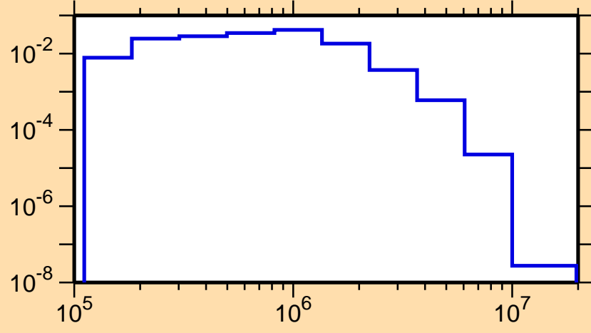
\sigma vs. E for ^{122}\text{In}(n,n_2)
