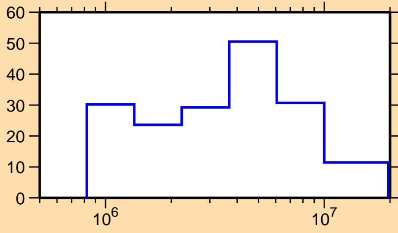
\Delta\sigma/\sigma vs. E for ^{122}\text{In}(n, el.)
