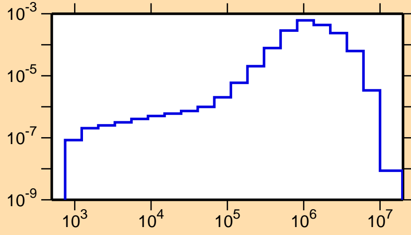
\sigma vs. E for ^{122}\text{In}(n,n_3)
