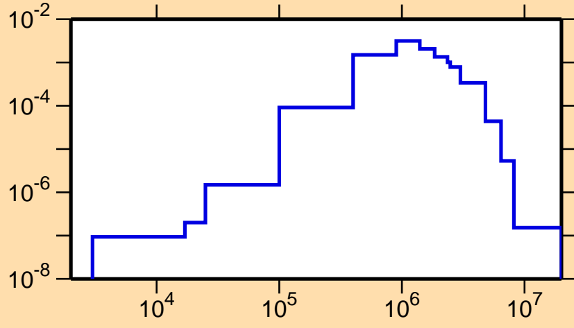
\sigma vs. E for ^{122}\text{In}(n,n_4)
