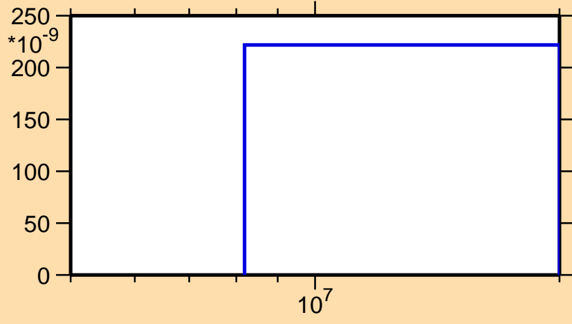
\sigma vs. E for ^{122}\text{In}(n,n\alpha)
