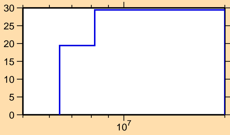
\Delta\sigma/\sigma vs. E for ^{123}\text{In}(n,el.)
