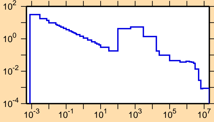
\sigma vs. E for ^{123}\text{In}(n,\gamma)
