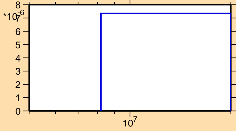
\sigma vs. E for ^{123}\text{In}(n,\alpha)
