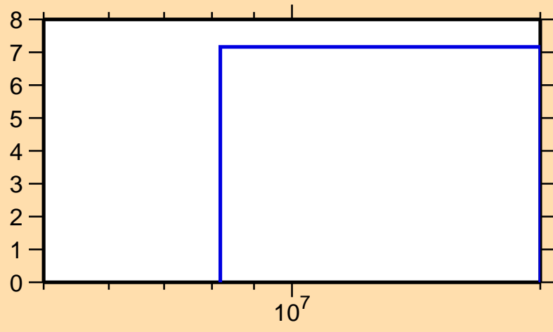
\Delta\sigma/\sigma vs. E for ^{123}\text{In}(n,\text{nonel.})
