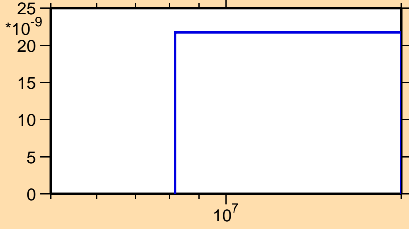
\sigma vs. E for ^{123}\text{In}(n,n\alpha)
