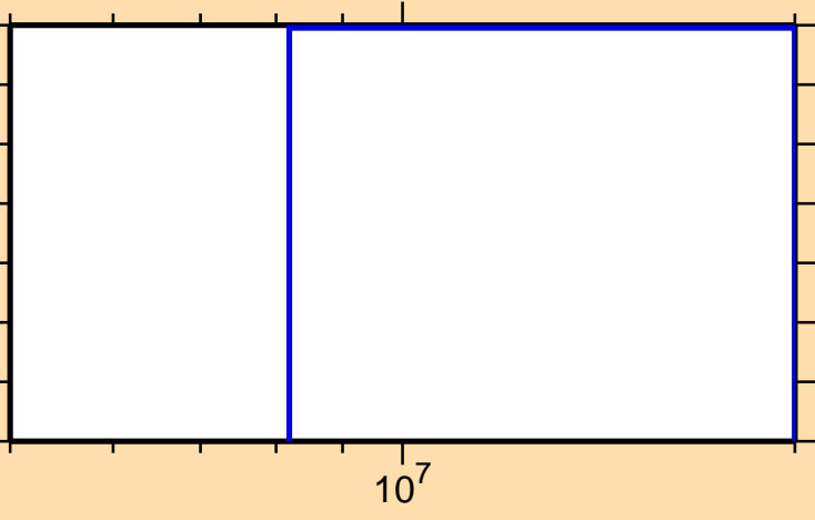
\sigma vs. E for ^{124}\text{In}(n,np)
