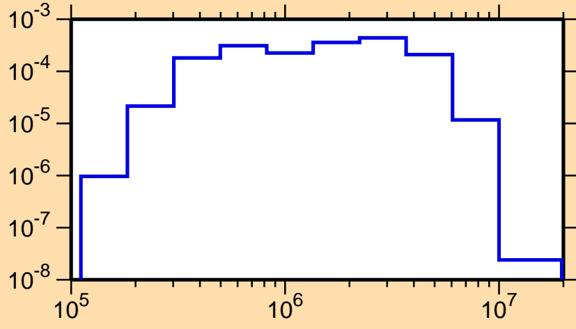
\sigma vs. E for ^{124}\text{In}(n,n_3)
