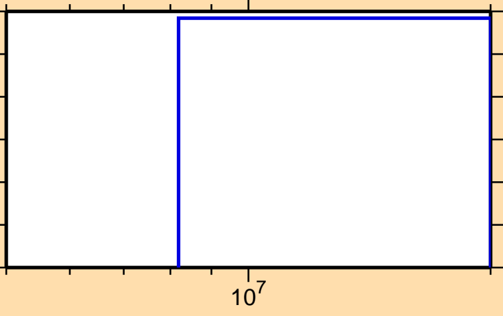
\sigma vs. E for ^{124}\text{In}(n,3n)
