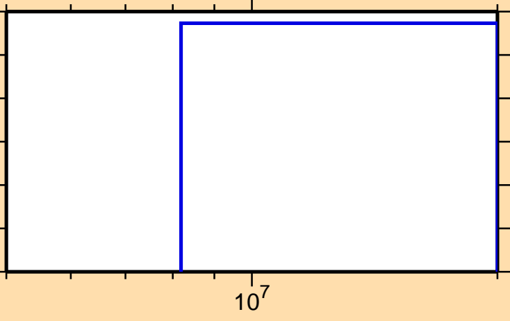
\sigma vs. E for ^{124}\text{In}(n,d)
