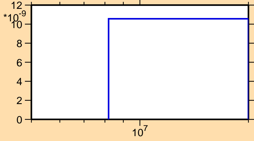
\sigma vs. E for ^{124}\text{In}(n,n\alpha)
