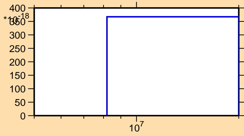
\sigma vs. E for ^{124}\text{In}(n,2n\alpha)
