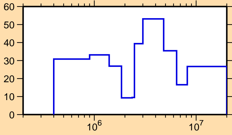
\Delta\sigma/\sigma vs. E for ^{124}\text{In}(n, el.)
