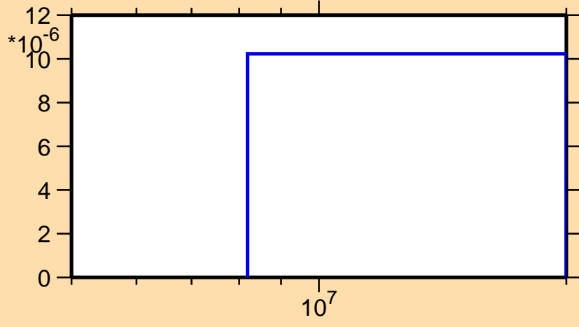
\sigma vs. E for ^{124}\text{In}(n,np)
