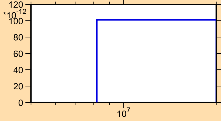
\sigma vs. E for ^{124}\text{In}(n,nt)
