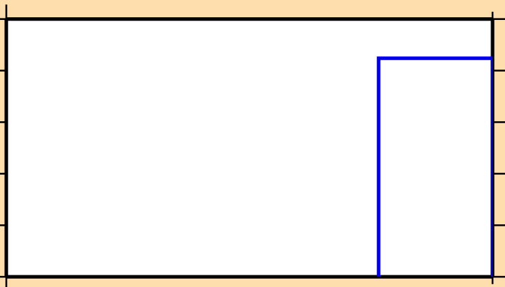
\sigma vs. E for ^{125}\text{In}(n,2np)
