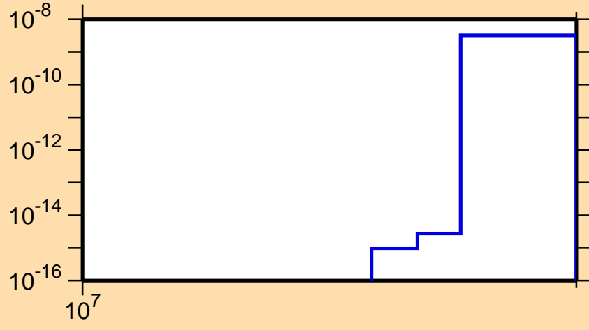
\sigma vs. E for ^{125}\text{In}(n,nt)
