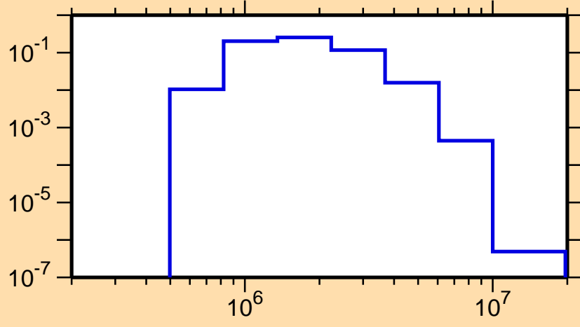
\sigma vs. E for ^{125}\text{In}(n,n_4)
