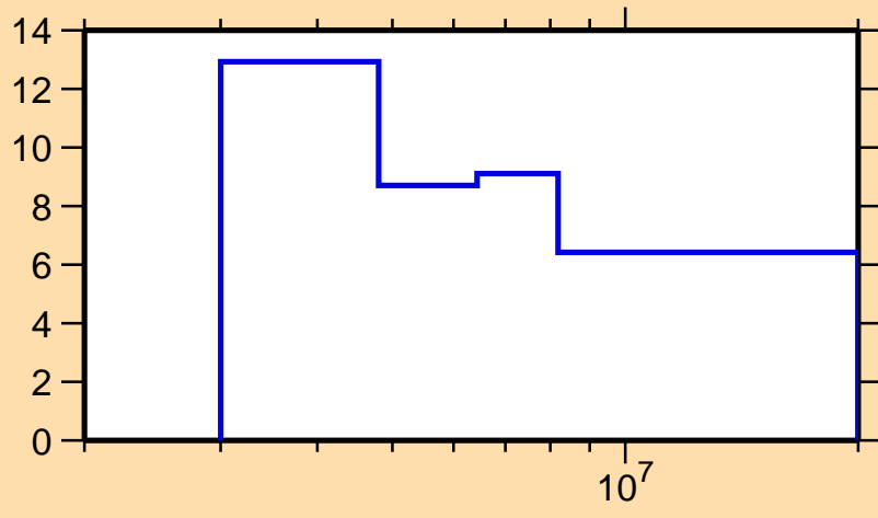
\Delta\sigma/\sigma vs. E for ^{127}\text{In}(n, n_{\text{onrel}})
