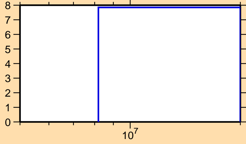
\Delta\sigma/\sigma vs. E for ^{127}\text{In}(n,\text{el.})
