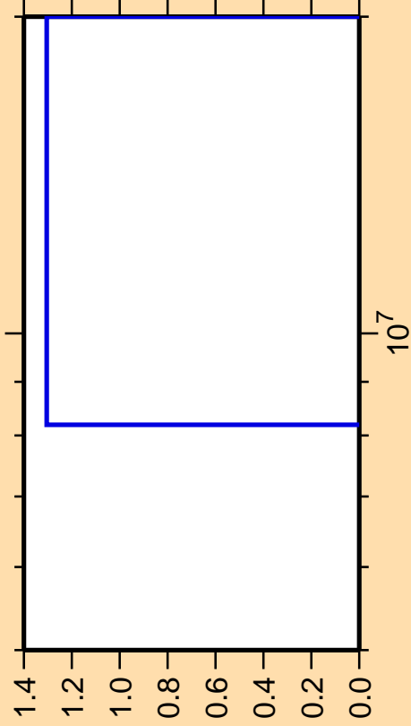
\Delta\sigma/\sigma vs. E for ^{127}\text{In}(n,nd)
