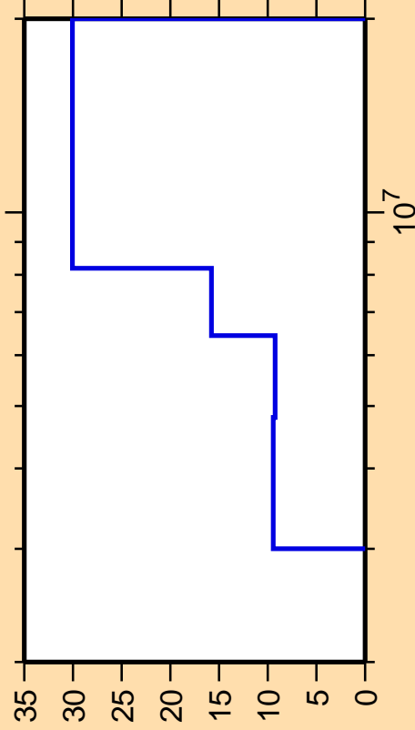
\Delta\sigma/\sigma vs. E for ^{127}\text{In}(n,n\text{cont.})
