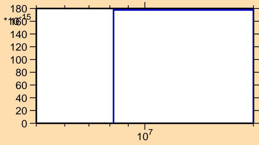
\sigma vs. E for ^{127}\text{In}(n,nd)
