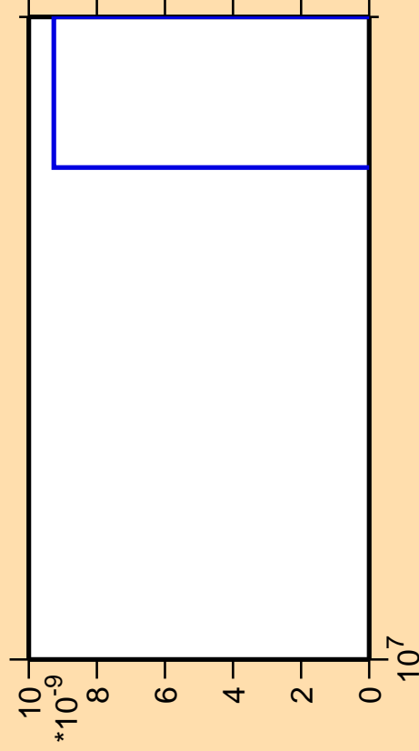
\Delta\sigma/\sigma vs. E for ^{127}\text{In} (mt 11)
