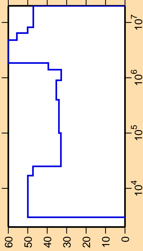
\Delta\sigma/\sigma vs. E for ^{127}\text{In}(n,n_4)
