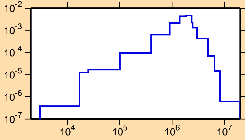
\sigma vs. E for ^{127}\text{In}(n,n_4)
